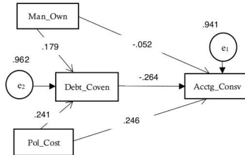
Figure 1. Path Analysis Result
