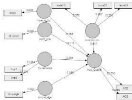
Figure 3. Inner Model Test (Equation Model)
