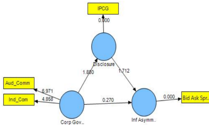
Figure 3. Inner Model Test
