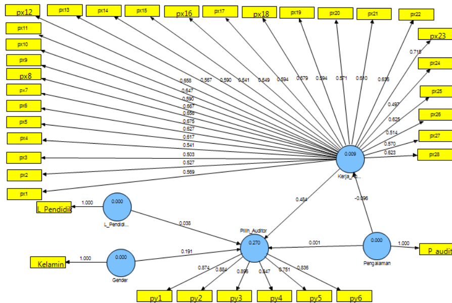
Gambar 1 Initial Outer Model Test
