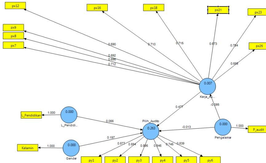
Gambar 2 Final Outer Model Test
